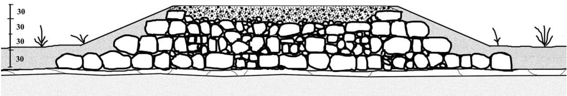
Figure 17, Structure of the roadbed of the road from Italia to Hispania in Hurones (Burgos) www.viasromanas.net
